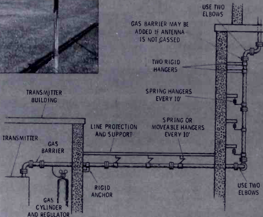
Fig. 1 Typical right line installation plan. It need not be to scale, but all necessary items should be shown and their positions in line.
