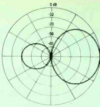
Fig. 3 Horizontal pattern of a 5-element yagi.
